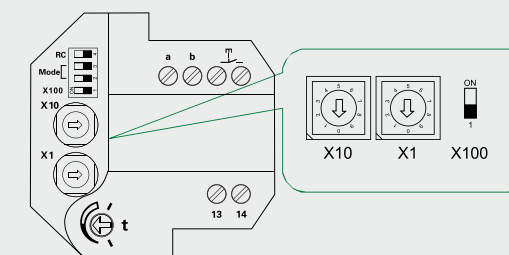
Setting address of switch actuator
