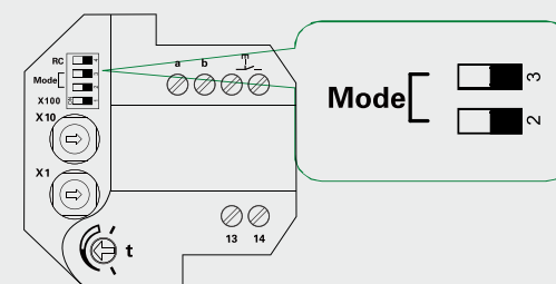
Setting mode of switch actuator
