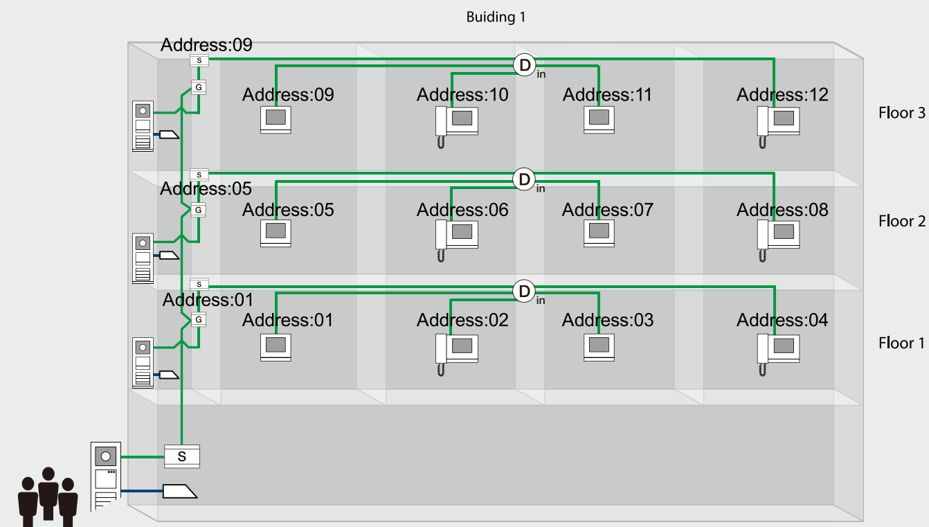
Setting address of floor gateway
