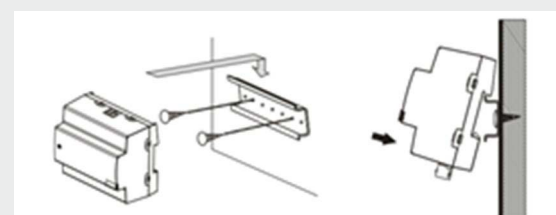
Mounting of the MDRC devices
