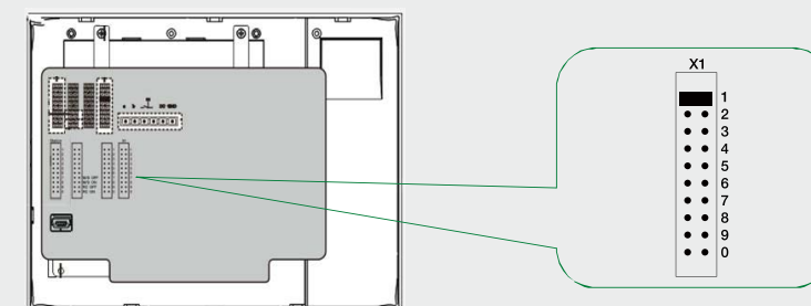
Setting the address of guard unit
